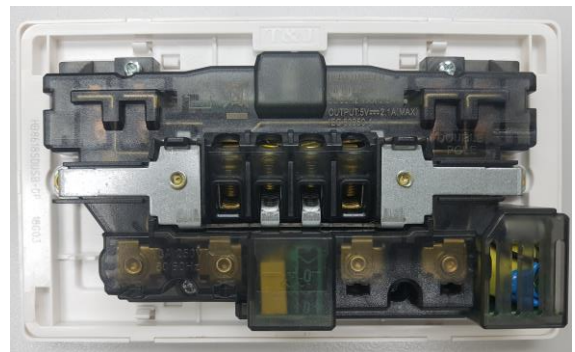
Back View of HB8618SDUSB-DP
