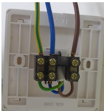
Sample wiring connection (with wire ferrules)
