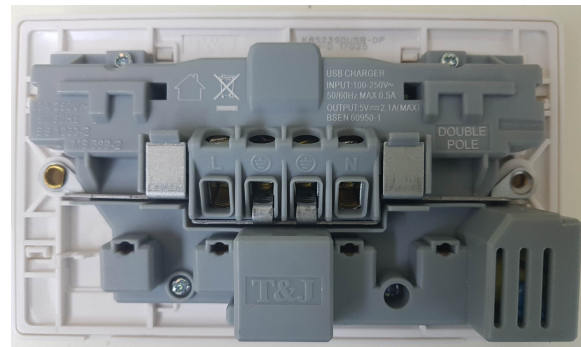
Back View of K8523SDUSB-DP
