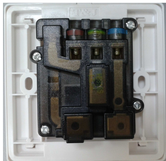
Back View of HB818S
