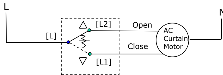
Connection Diagram for W2222 (Retractive Switch)
