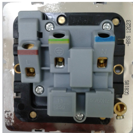
Back View of GC818S
