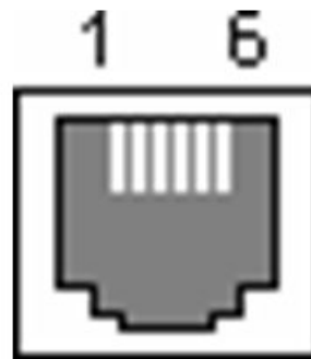
pin assignment F99018 (RJ 11 jack)
