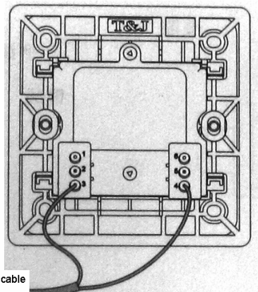
2 wire telephone circuit
