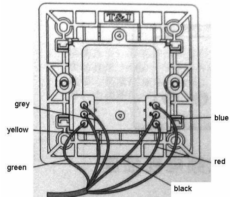
6 wire telephone circuit
