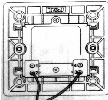
2 wire telephone circuit
