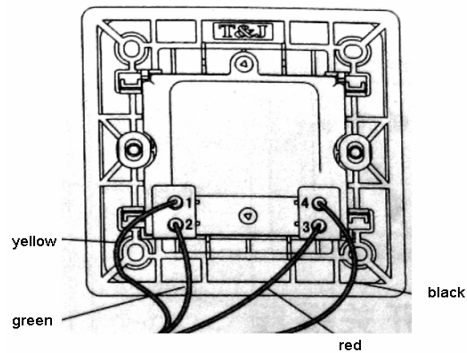
4 wire telephone circuit
