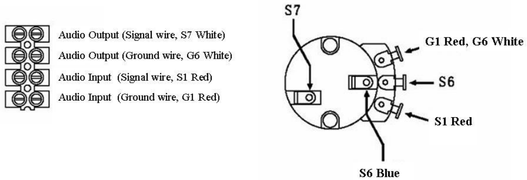
Terminal on K2-V
